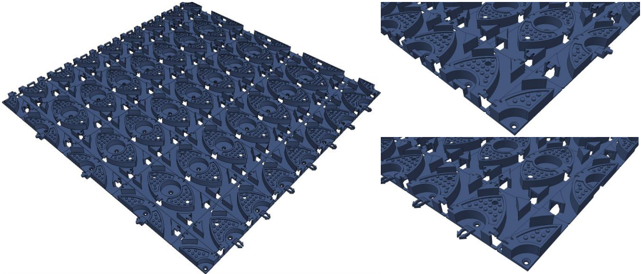
600mm x 600mm TechnoLo Low Profile Underfloor Heating Panel
